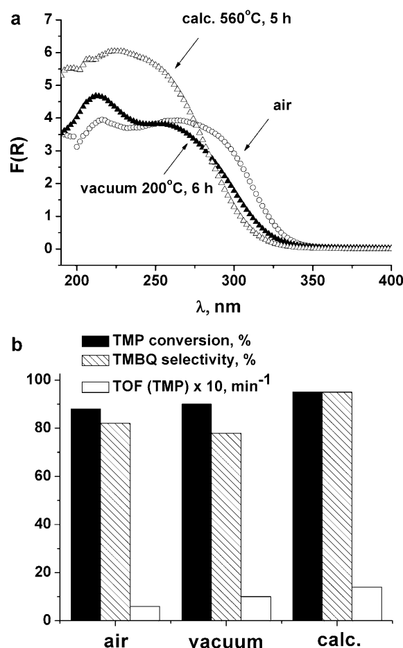
Figure 4. The effect of different treatments on the DR-UV spectrum a ) and catalytic performance b ) of Ti/SiO 2 (Davicat, 1.93 wt% Ti).
