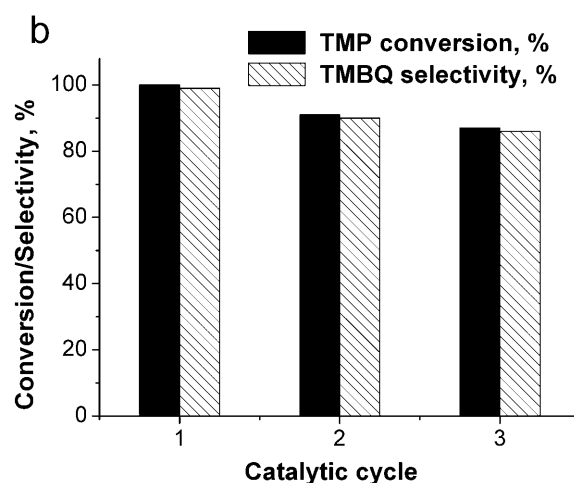
Figure 6. Catalyst recycling in TMP oxidation with 30% \text{H}_2\text{O}_2 over \text{Ti}/\text{SiO}_2 (Nippon–Kasei): a) Ti 2.09 wt% and b) Ti 3.63 wt%.
