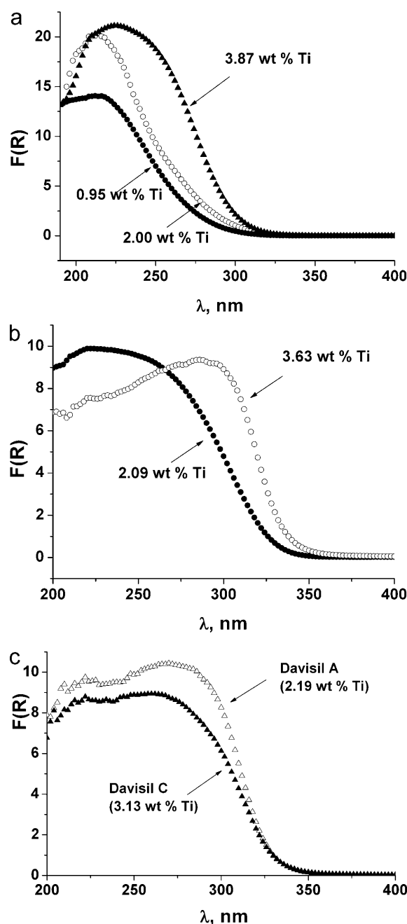
Figure 1. DR-UV spectra of Ti catalysts prepared by grafting Ti(Cp) 2 Cl 2 on a) MCM-41, b) Nippon-Kasei silica and c) Davisil silicas.
